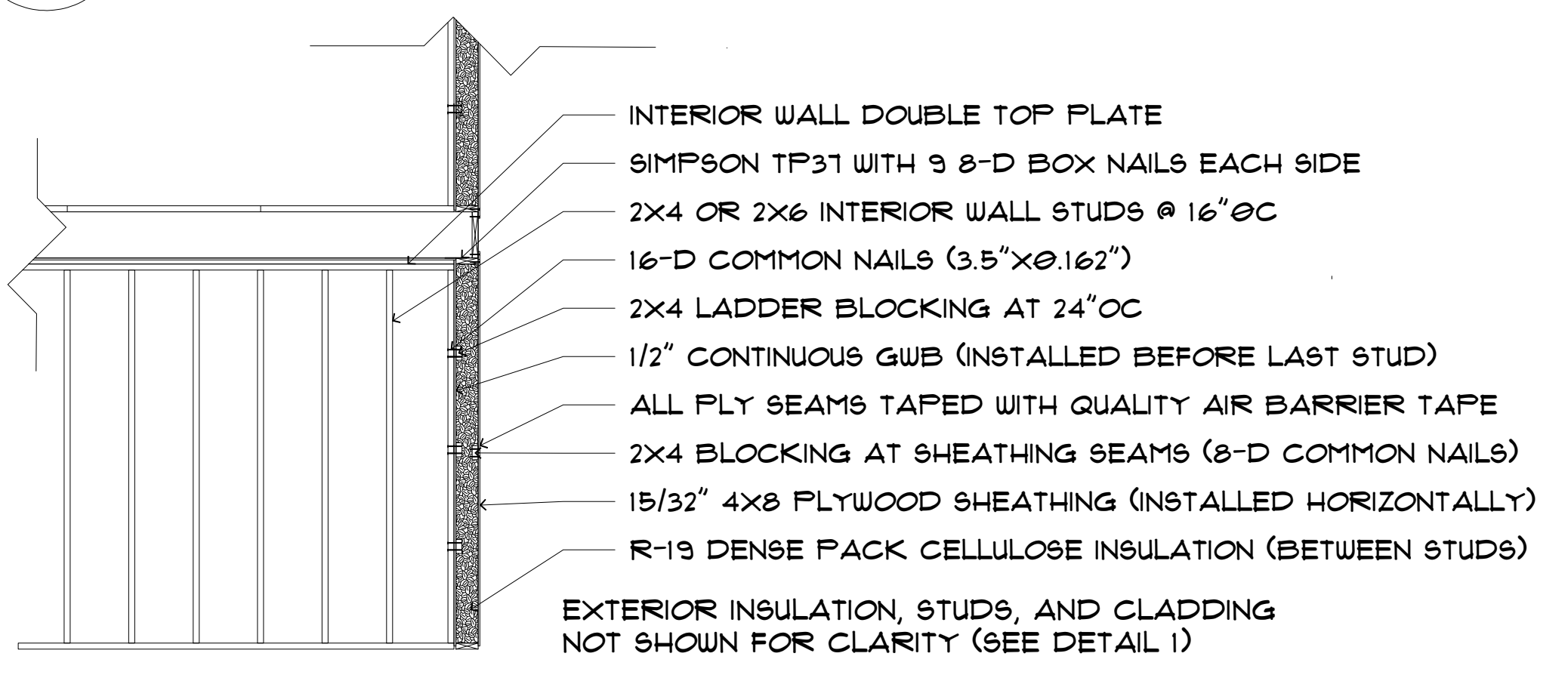
3 INTERIOR TO EXTERIOR
