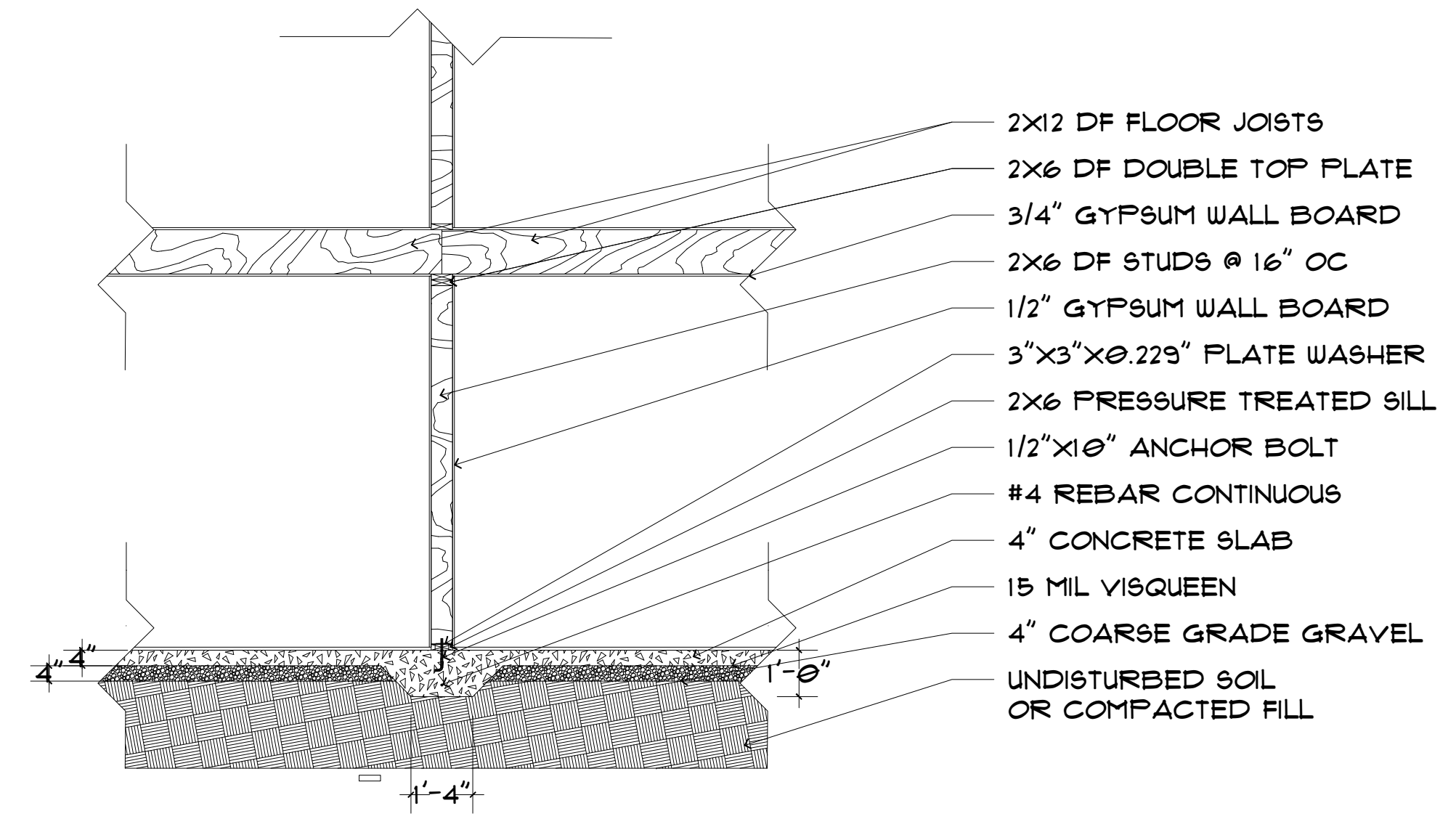
2 INTERIOR BEARING WALL
