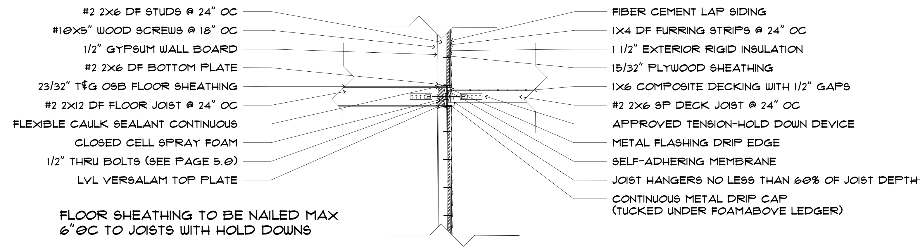
4 DECK ATTACHMENT DETAIL
