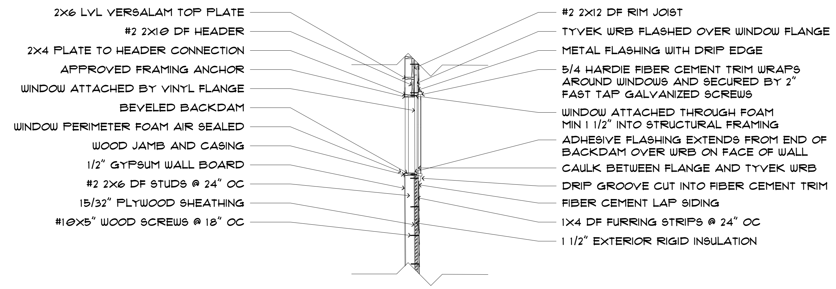
5 EXTERIOR CORNER DETAIL
